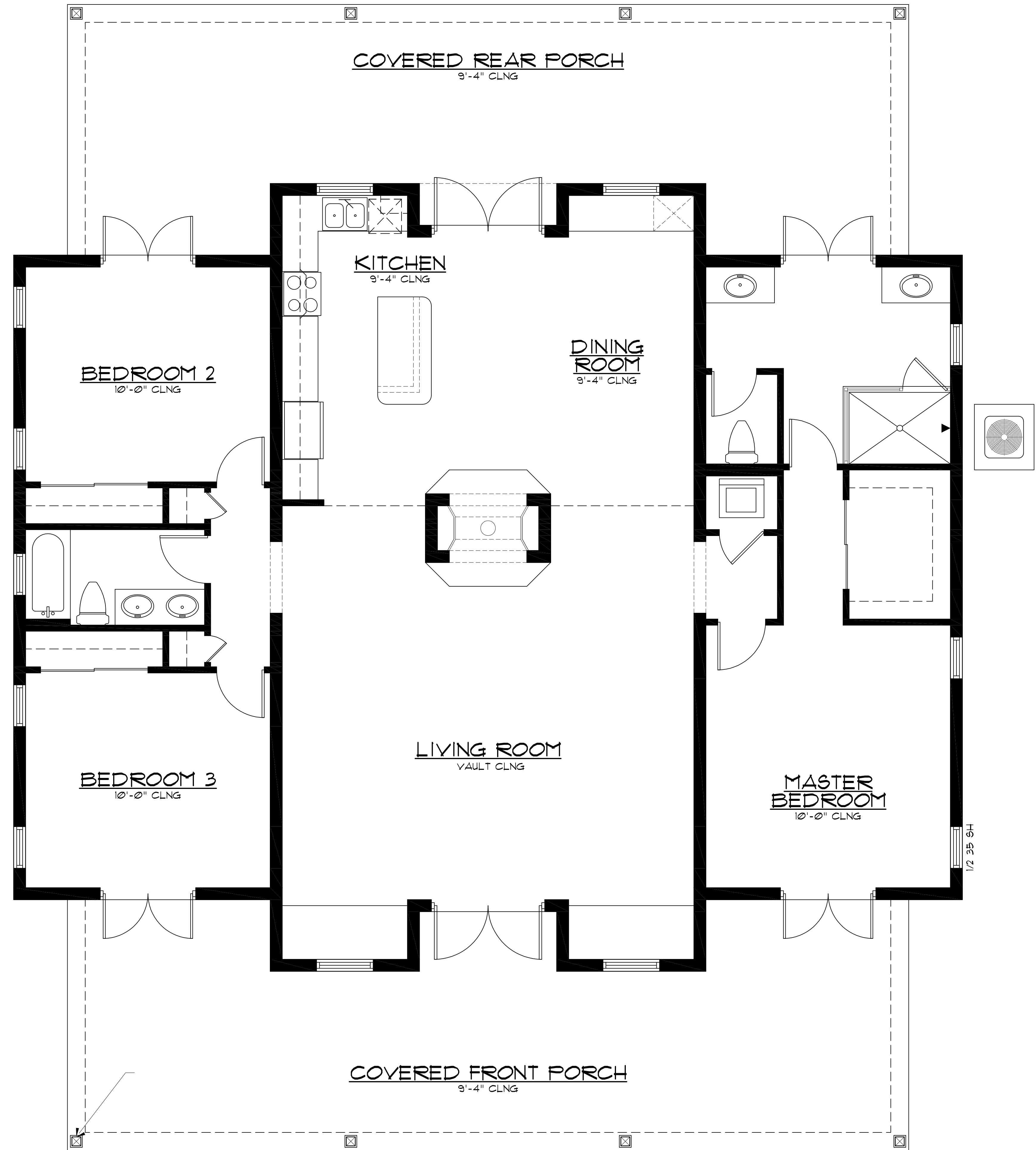
LAKE COTTAGE LOT 12 FLOOR PLAN
