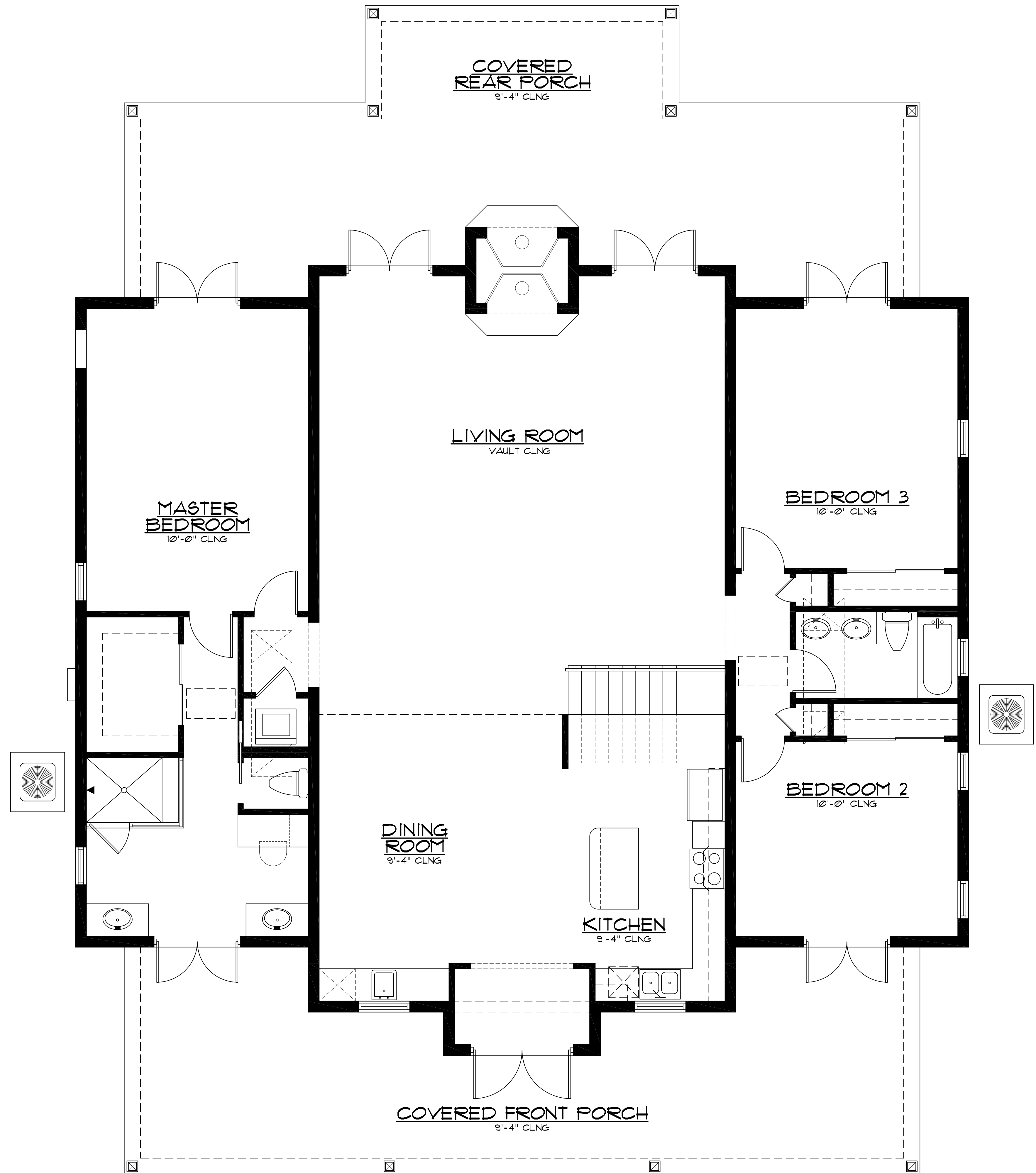
LAKE COTTAGE LOT 21 FLOOR PLAN
