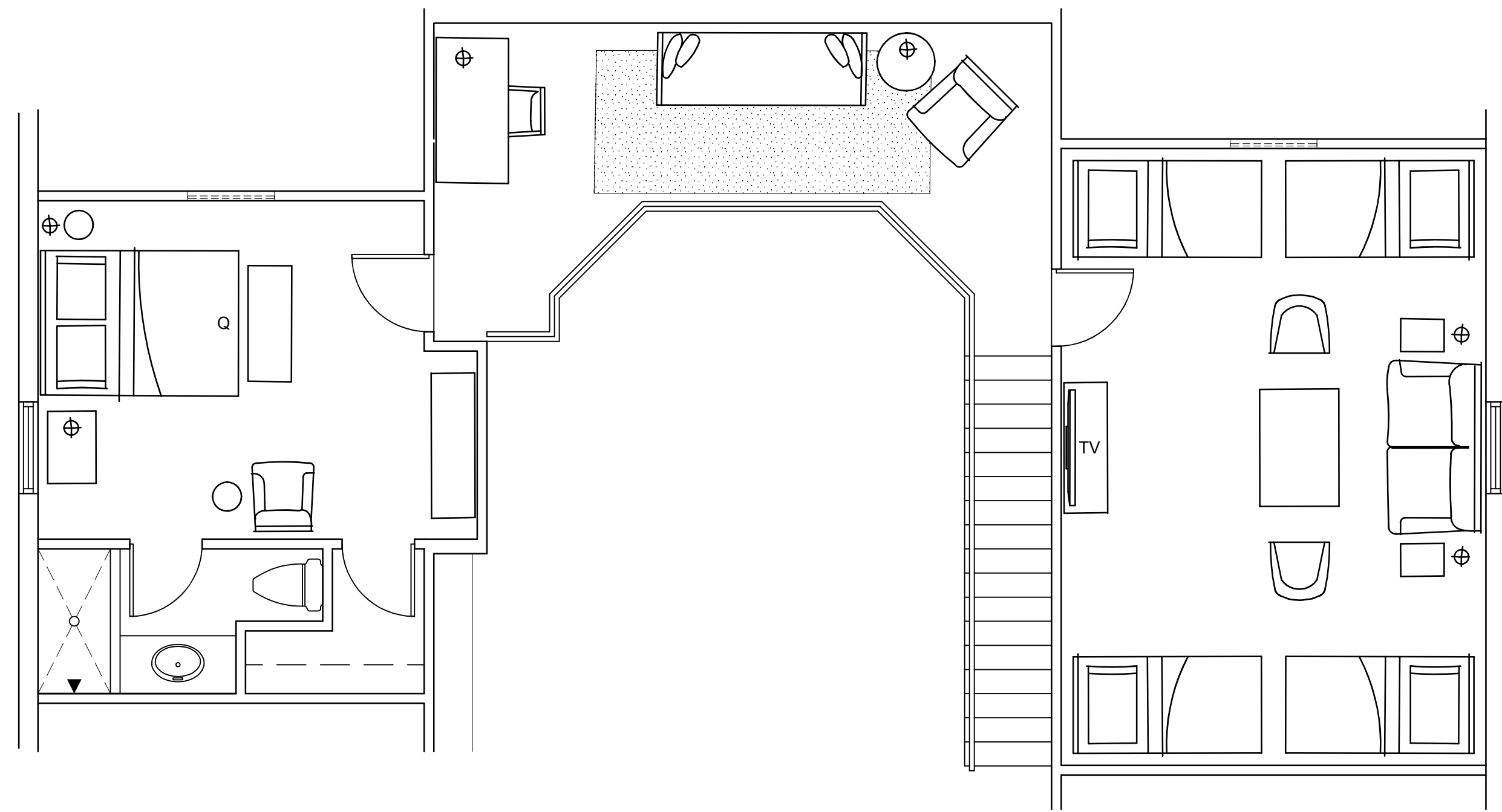
LOFT FURNITURE PLAN SCALE: 1/4" = 1'-0"
